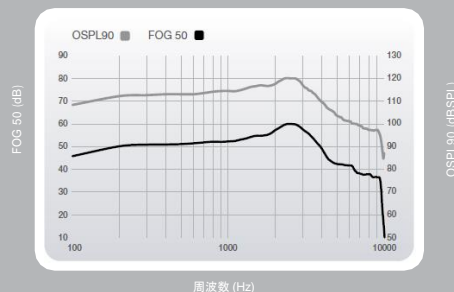
Muse micro RIC 312 (60 ゲイン)
