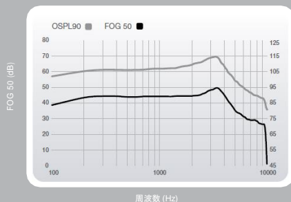
Muse micro RIC 312 (50 ゲイン)
