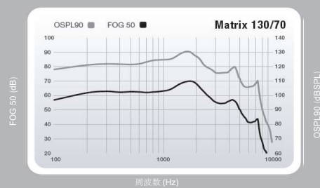
Muse iQ RIC 312 AP (70 ゲイン)
