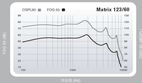
Muse iQ RIC 312 AP (60 ゲイン)
